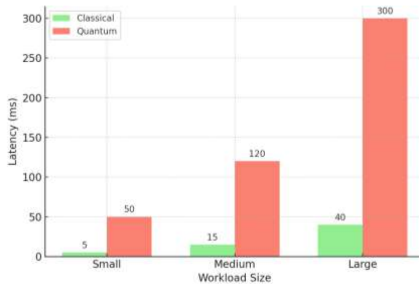
Figure 2. Latency Comparison Between Classical and Quantum
