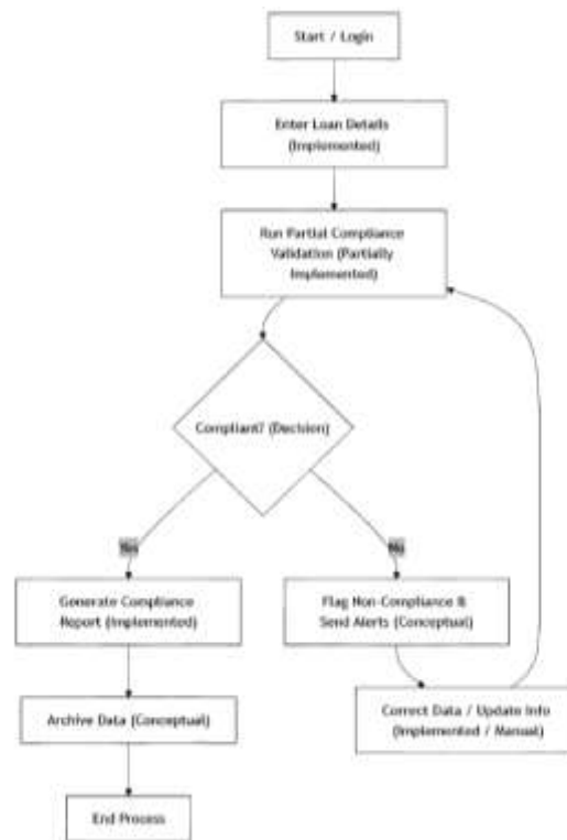
Figure 2. Compliance Verification Workflow in FinTrack
