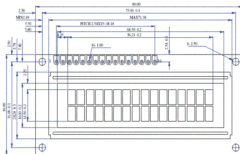
Figure 2. General Pin Diagram of LCD
