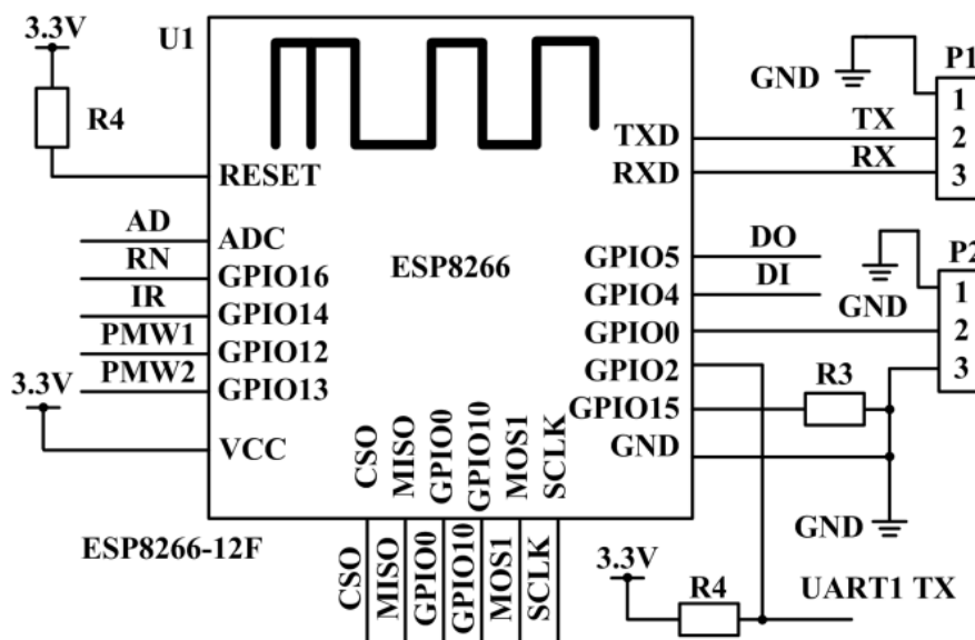
Figure 3. General NodeMCU ESP8266
