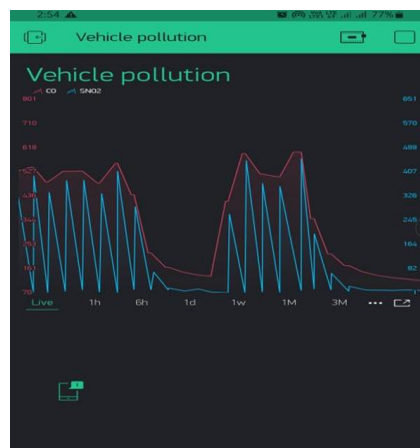
Figure 10. Result Displayed in Smart Mobile
