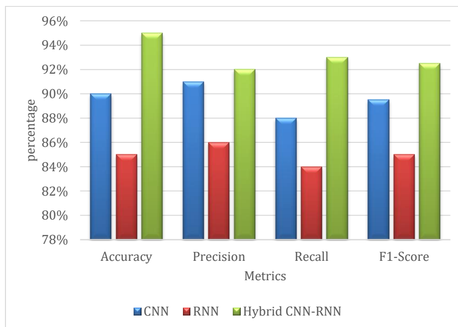
Figure 2. Model Performance
