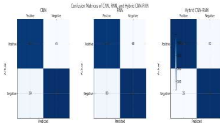
Figure 5. Confusion Matrices for CNN, RNN, and Hybrid CNN-RNN Models
