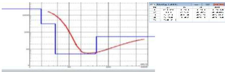
Figure 5: Resistivity sounding curve for Ukwa Comm
