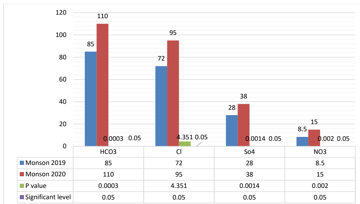
Figure 1. Comparison of Variability of Main Anions in the Musi River Basin during Monsoon Seasons (2019-2020): ANOVA Test Results
